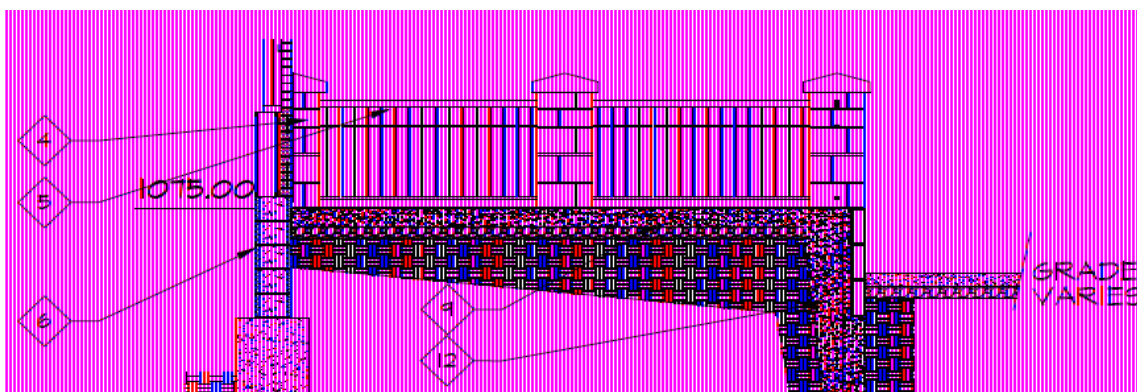
SECTION A
